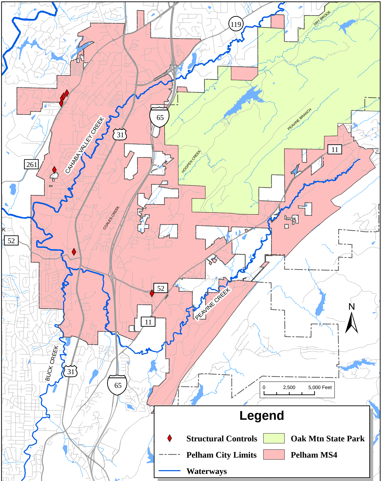
Figure 2: Structural Controls
